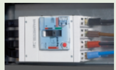
Use of a sleeve on a wired DPX 250
